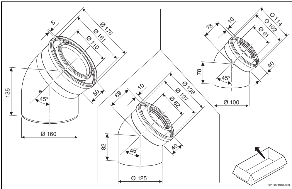
1 Ø 110/160: 7738113104/...3949, Ø 80/125: 7738112593, Ø 60/100: 7738112501 / ...2875 / ...3495
