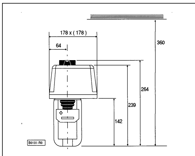
Abb. 4 ML6421A, ML7421A
